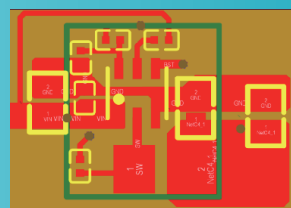
SCT2230B SOT563 20mm² solution size → 269W/cm³
