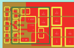
SCT2233M PPD Module™ 13mm² solution size → 381W/cm³
